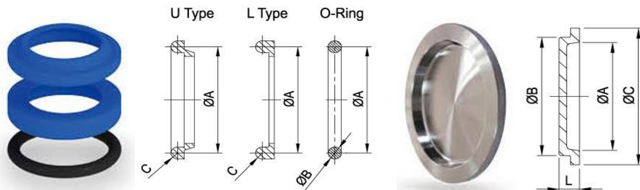
RJT Seal Ring (EPDM, Silicon, Viton)
