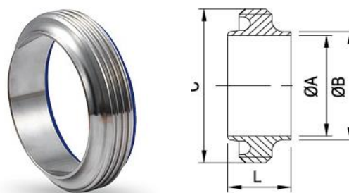
RJT Welding Male RJT-15
